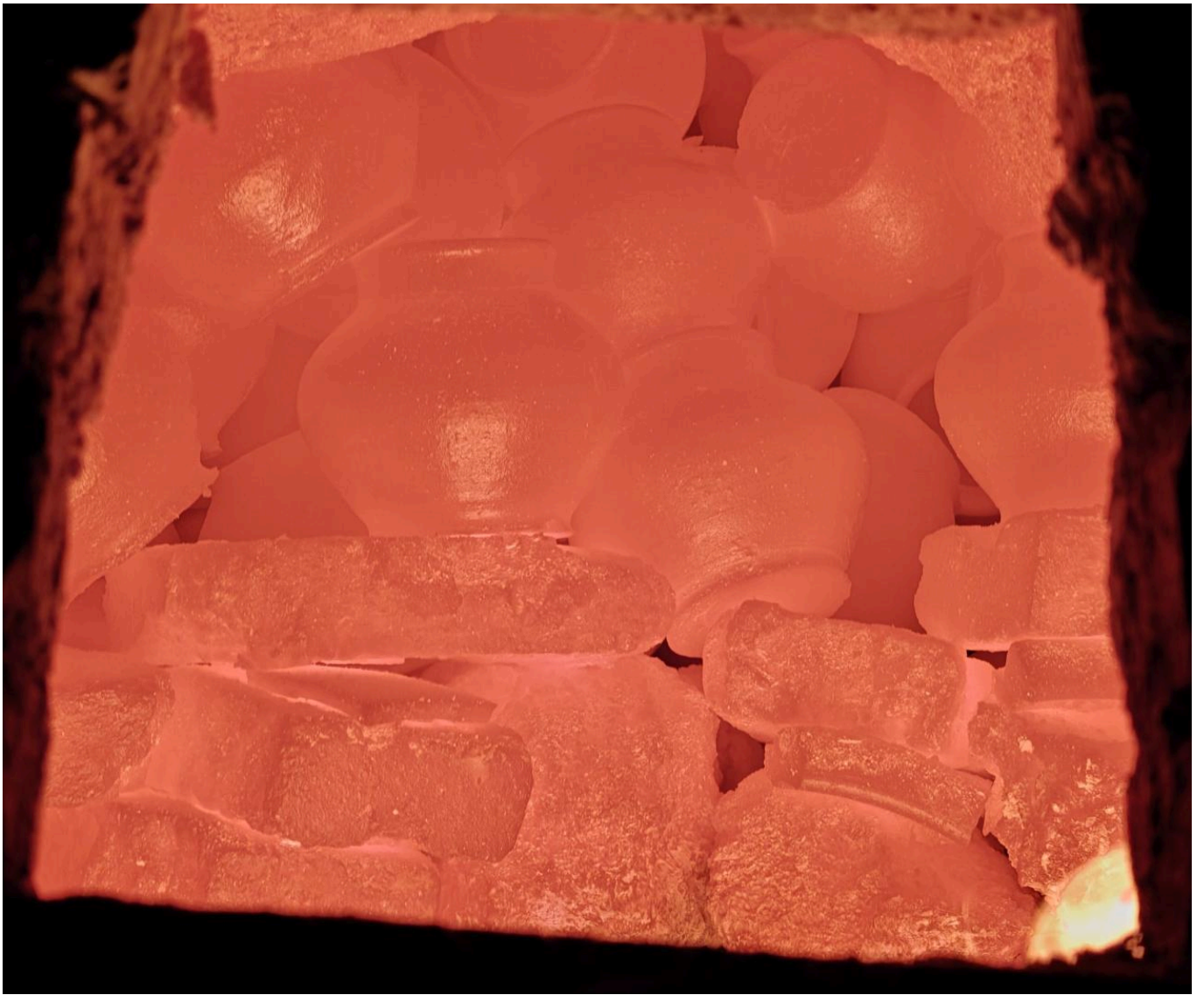
FIG 2. THE EXPERIMENTALLY RECONSTRUCTED POTTERY KILN IS FIRING POTTERY.. PHOTO BY BANGCHENG TANG
